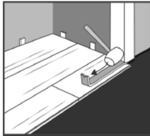
Step 2: Use rubber mallet and pull bar to lock this piece of flooring
