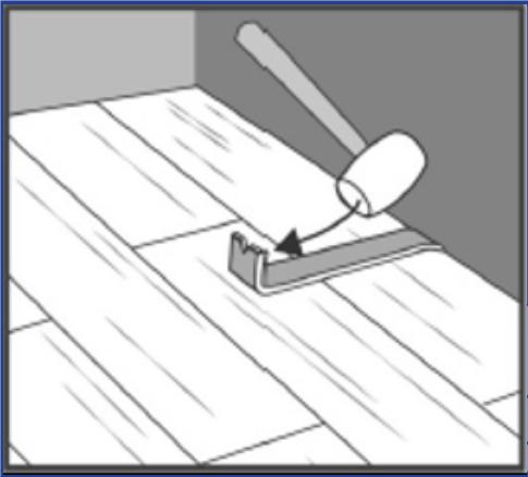
Step 9: Use rubber mallet and pull bar to lock long edges of flooring on final row.
